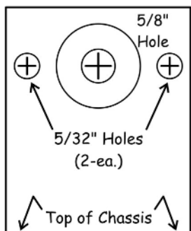
Full-Sized Drill Template
