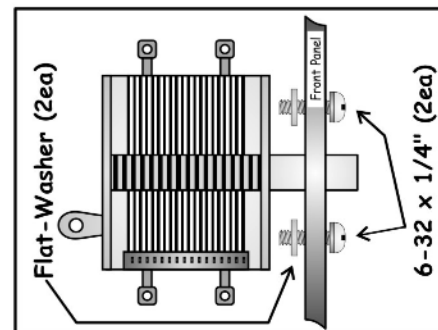
15-001, Variable Capacitor, Mounting to: 0.125" Front Panel
